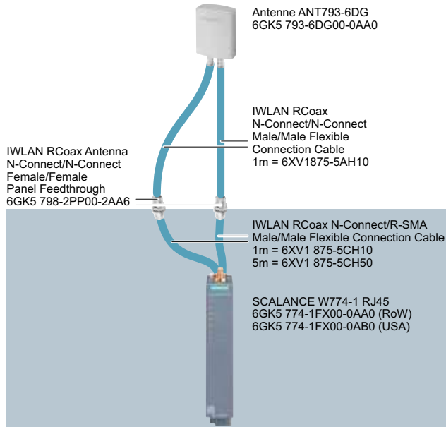
Control cabinet
